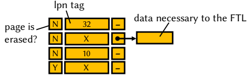
Figure 7: Emulated flash pages in VST.
