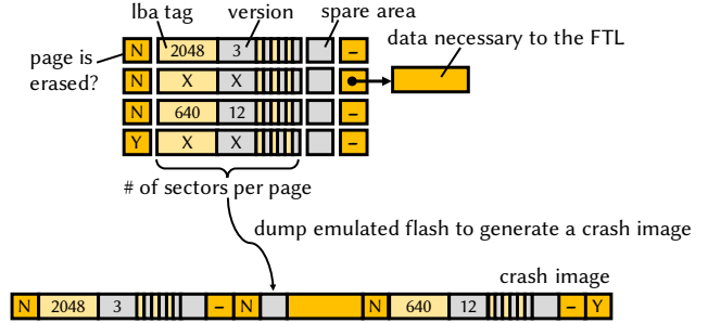
Figure 8: Extensions for crash-guarantee validation.
